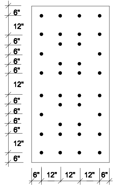
36 FASTENERS PER 4' x 8' BOARD
