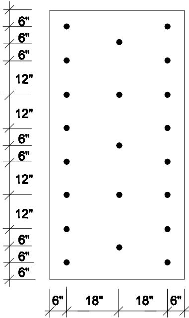
21 FASTENERS PER 4' x 8' BOARD
