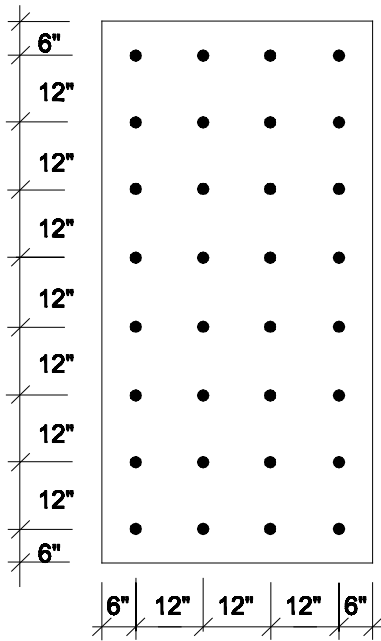
32 FASTENERS PER 4' x 8' BOARD
