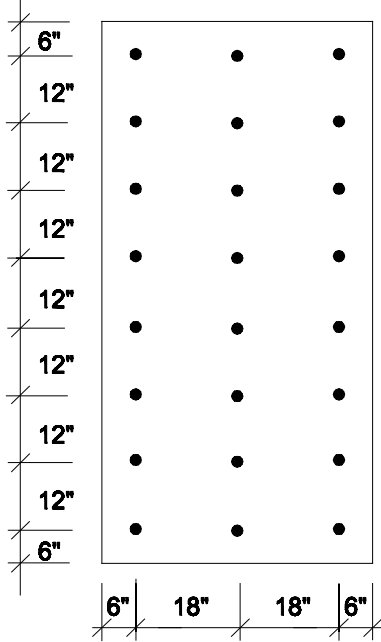
24 FASTENERS PER 4' x 8' BOARD
