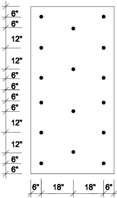
16 FASTENERS PER 4' x 8' BOARD
