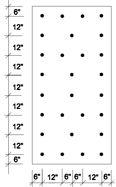
28 FASTENERS PER 4' x 8' BOARD
