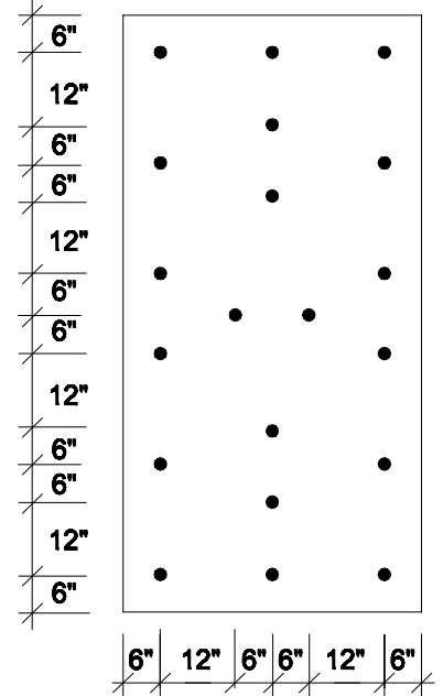
20 FASTENERS PER 4' x 8' BOARD
