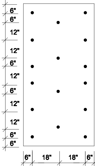
16 FASTENERS PER 4' x 8' BOARD
