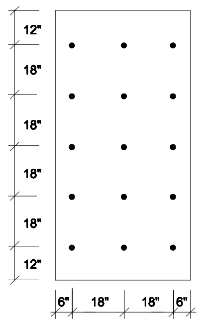
15 FASTENERS PER 4' x 8' BOARD
