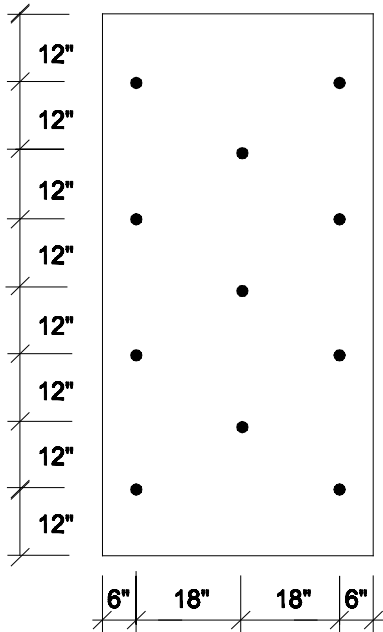
11 FASTENERS PER 4' x 8' BOARD
