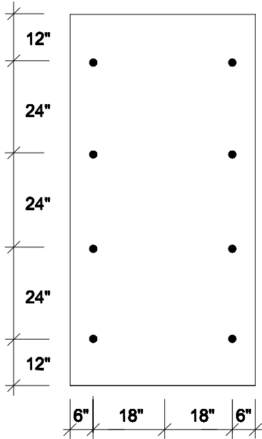
8 FASTENERS PER 4' x 8' BOARD
