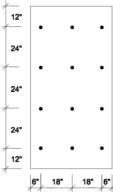
12 FASTENERS PER 4' x 8' BOARD
