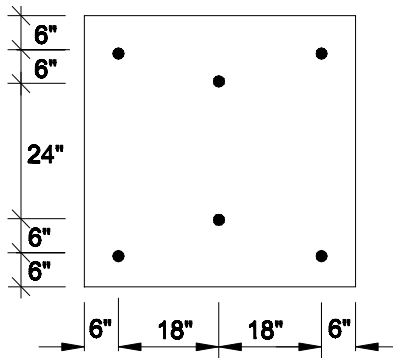
6 FASTENERS PER 4' x 4' BOARD
