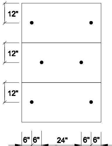
2-2-2 FASTENERS PER 2' x 4' SECTION
