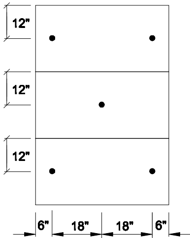
2-1-2 FASTENERS PER 2' x 4' SECTION
