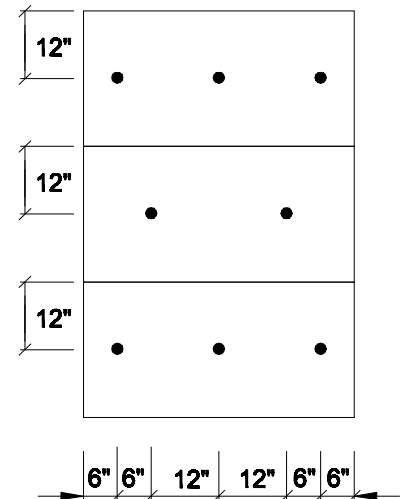
3-2-3 FASTENERS PER 2' x 4' SECTION
