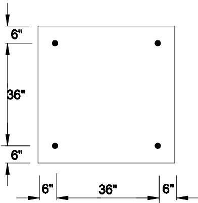
4 FASTENERS PER 4' x 4' BOARD
