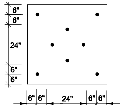
8 FASTENERS PER 4' x 4' BOARD
