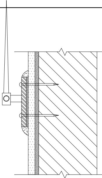
MOUNTING SECTION
