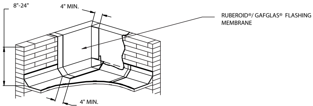
INSIDE CORNER "FOOTBALL" REINFORCEMENT PATCH
