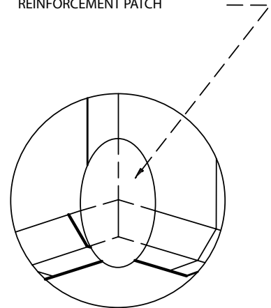
INSIDE CORNER "FOOTBALL" REINFORCEMENT PATCH
