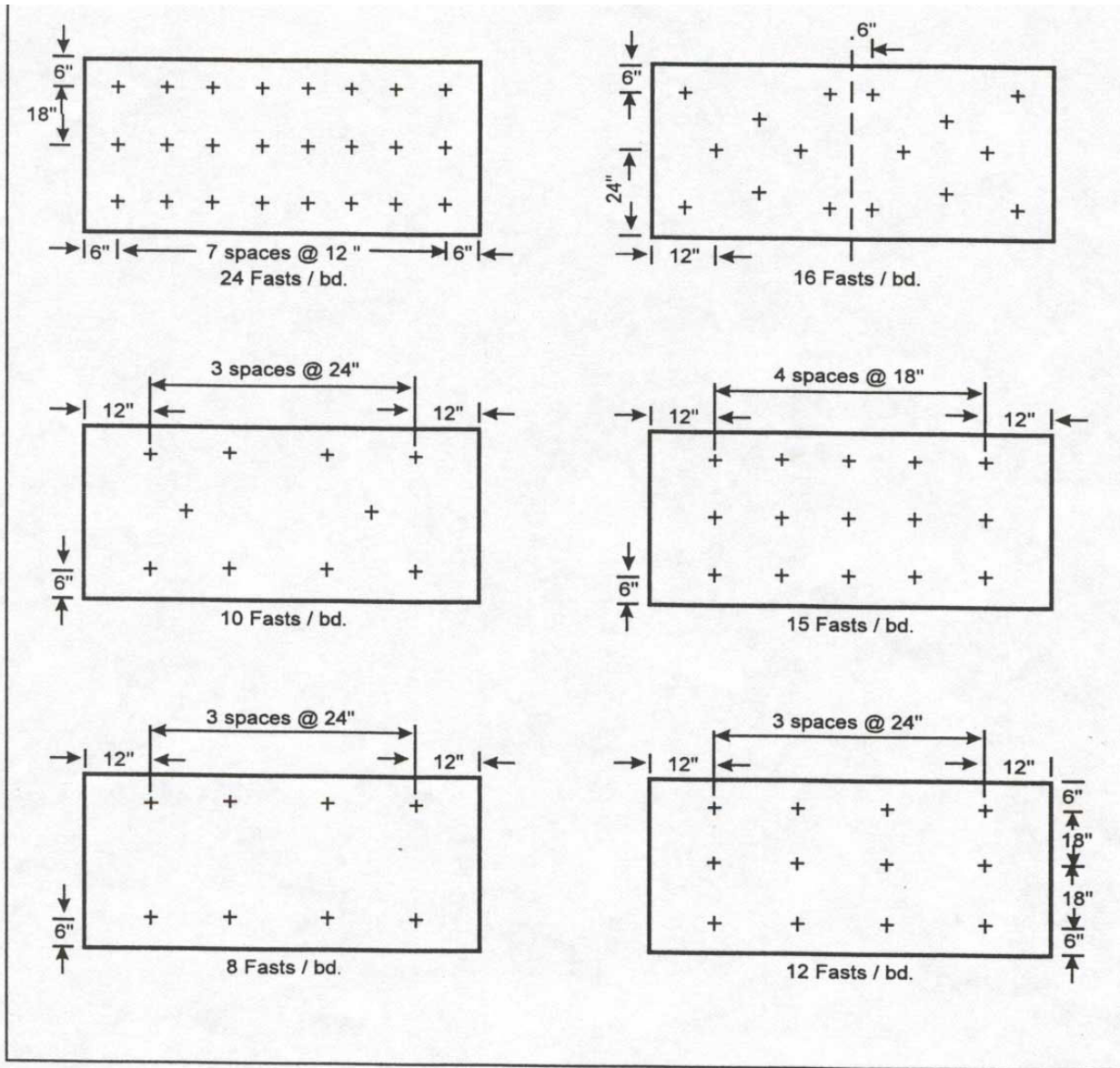
Fig. 6. Fastener placement 4 x 8 ft (1.2 x 2.4 m) boards.
