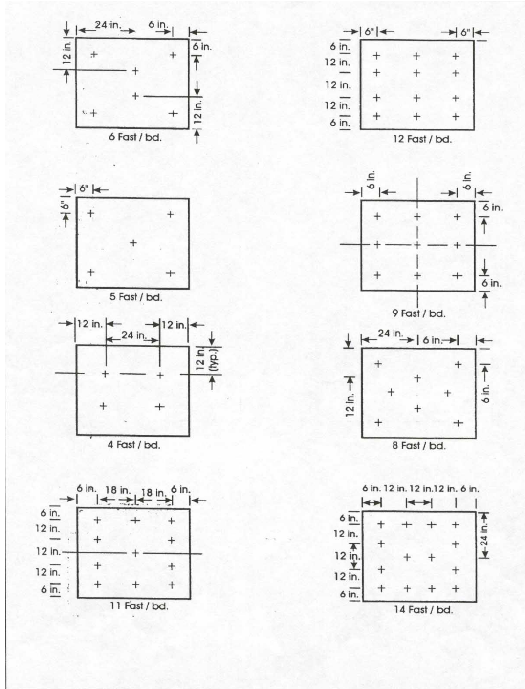
Fig. 5. Fastener placement 4 x 4 ft (1.2 x 1.2 m) boards.
