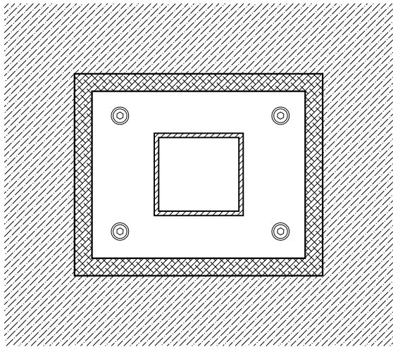
ENLARGED PLAN VIEW OF RAILING POST
