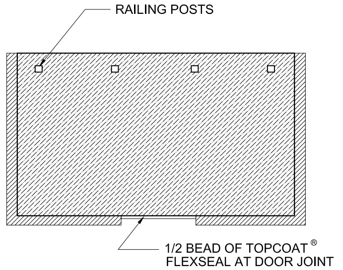
PLAN VIEW OF BALCONY
