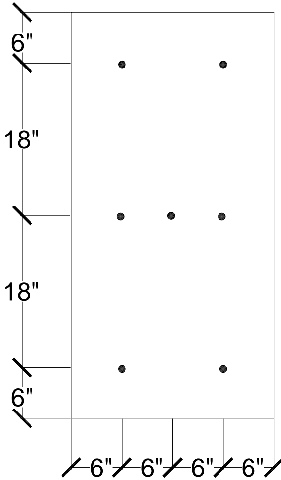
7 FASTENERS PER 2' x 4' BOARD
