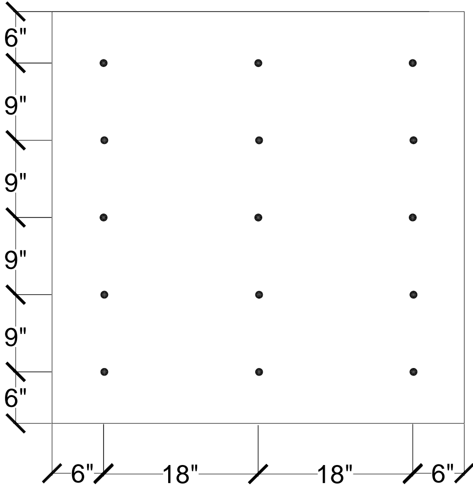
15 FASTENERS PER 4' x 4' BOARD
